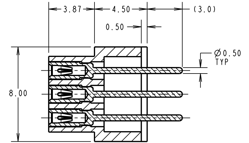
SECTION Y-Y
