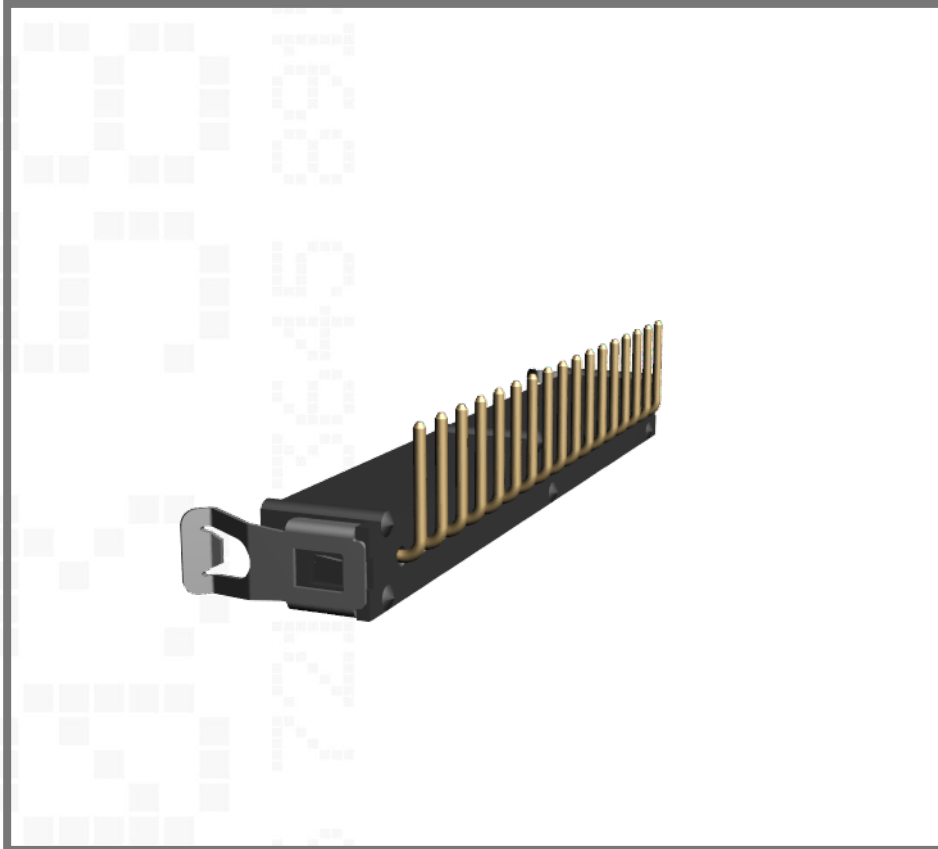
Single row, Locking Latch, 3mm tail, Gold, 17 contacts
