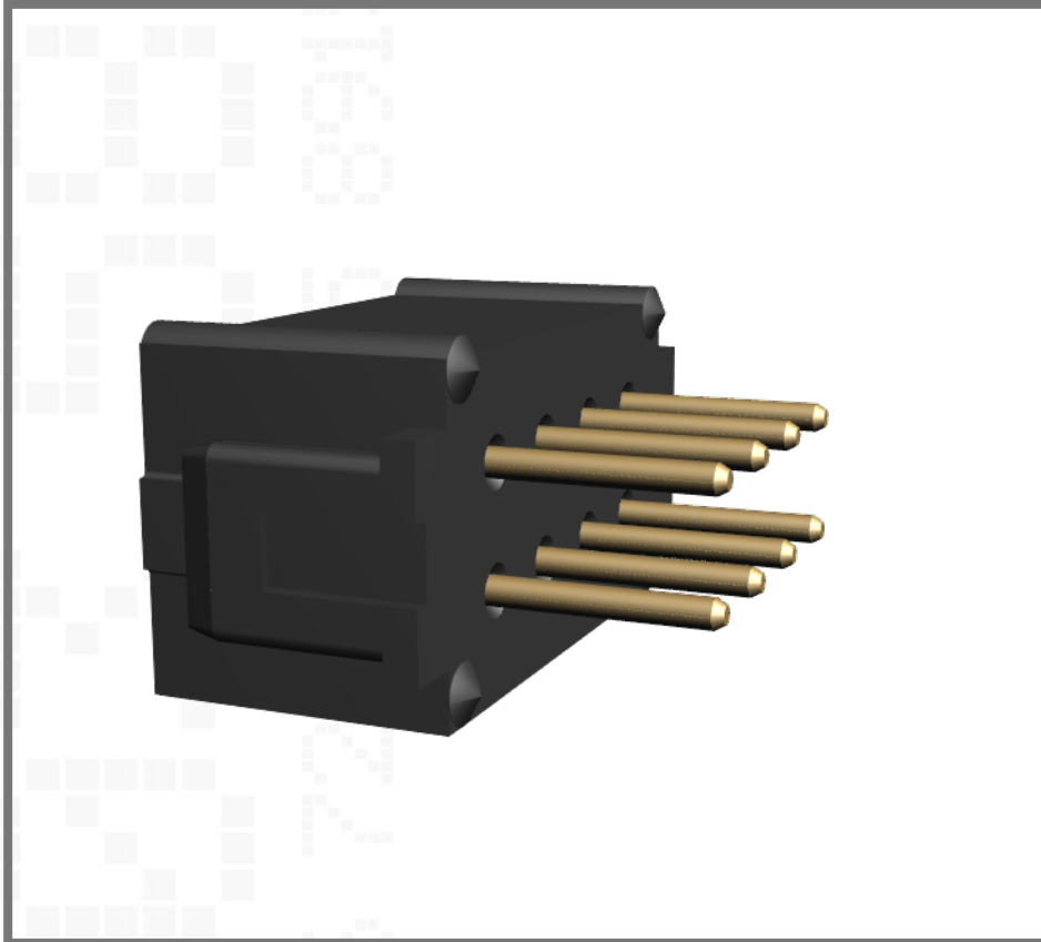
Double row, Unlatched, 3mm tail, Gold, 4+4 contacts
