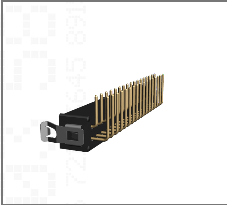
Double row, Locking Latch, 3mm tail, Gold, 17+17 contacts
