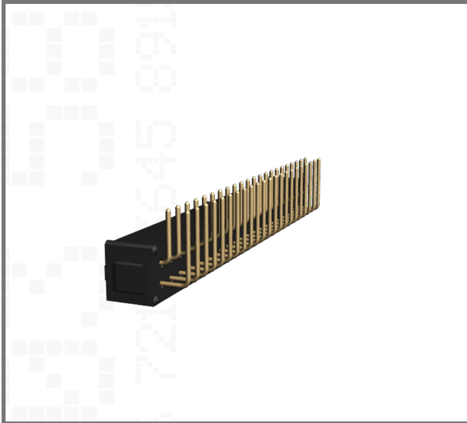
Double row, Unlatched, 3mm tail, Gold, 22+22 contacts
