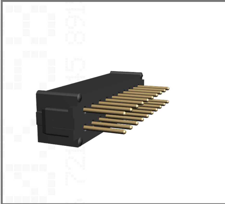
Double row, Unlatched, 4.5mm tail, Gold, 10+10 contacts
