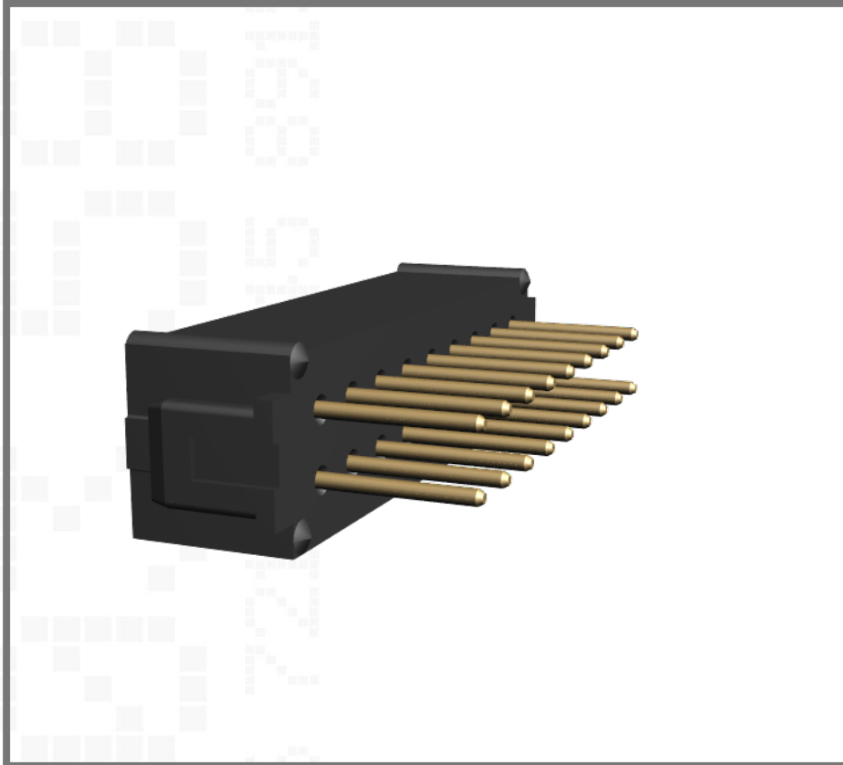
Double row, Unlatched, 4.5mm tail, Gold, 9+9 contacts
