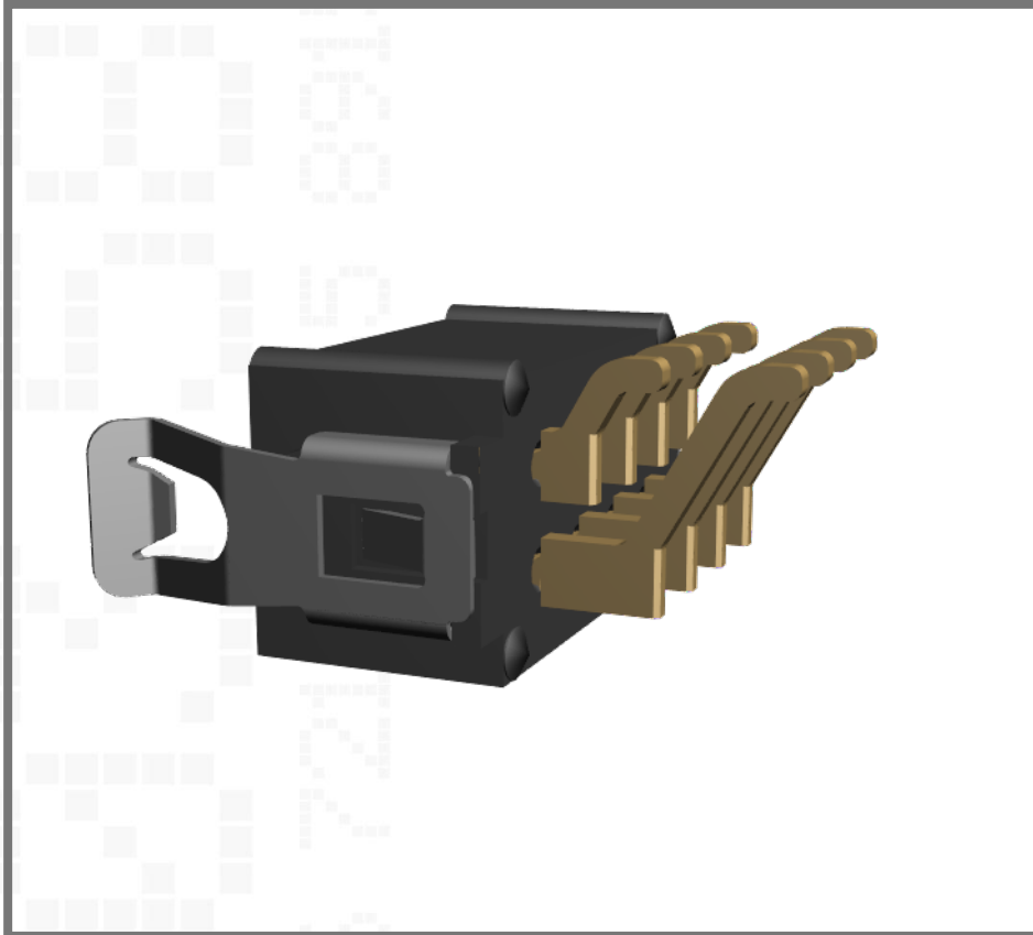
Double row, Locking Latch, Gold, 4+4 contacts
