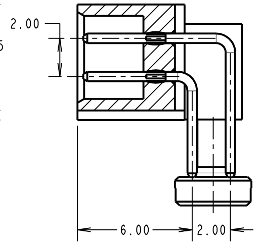
SECTION X-X
