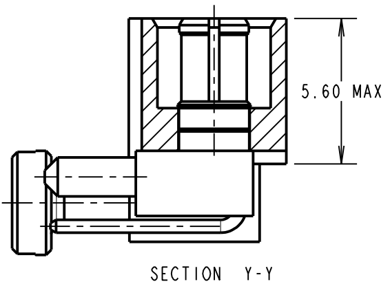
VIEW OF POWER CONTACT
