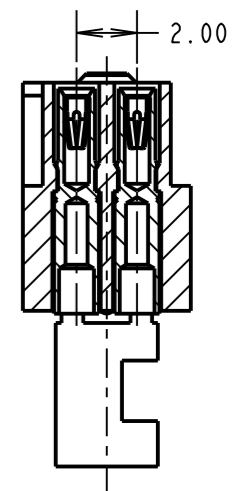
SECTION X-X
