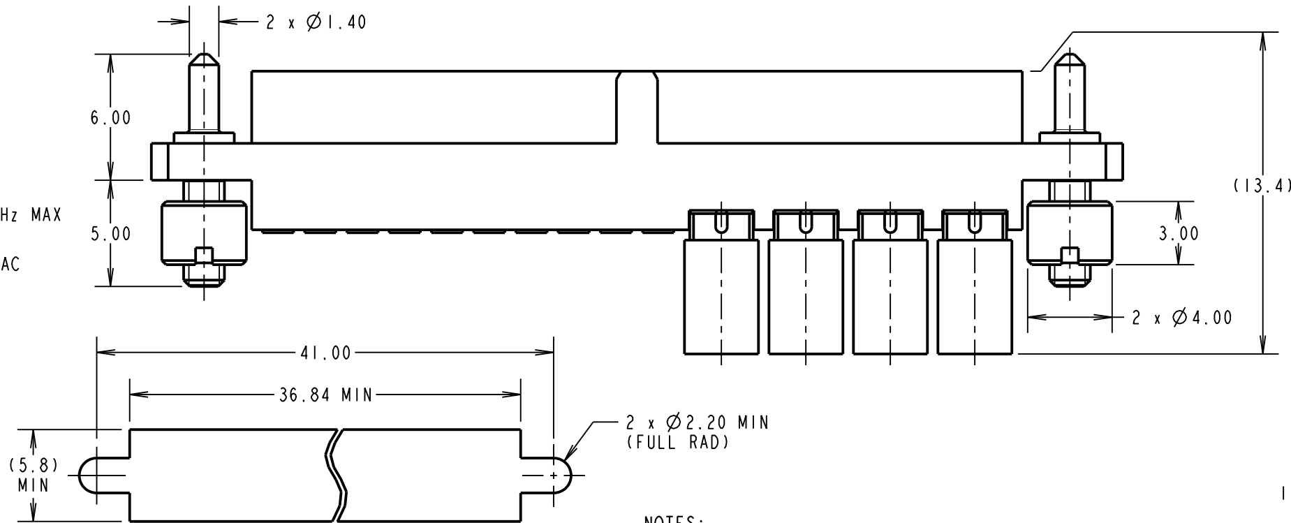
RECOMMENDED PANEL LAYOUT
