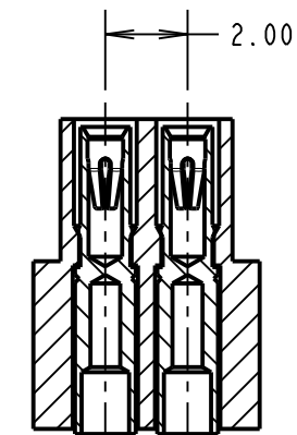
SECTION X-X
