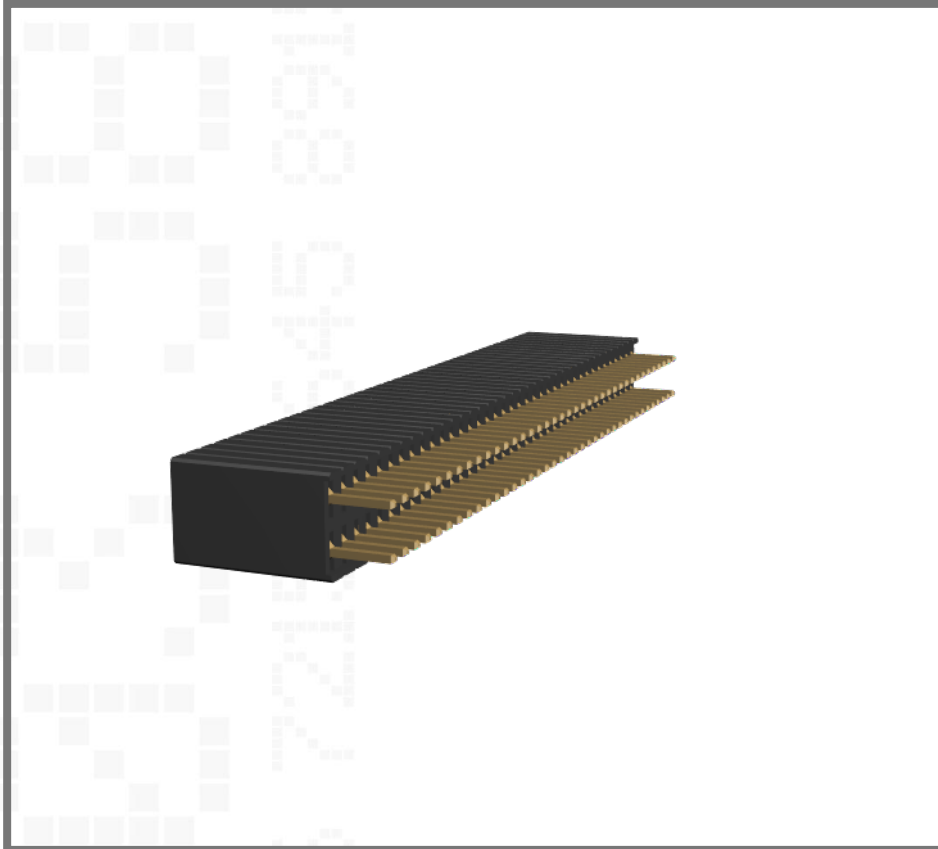
Dual row, 8.5mm high, gold, 38+38 contacts
