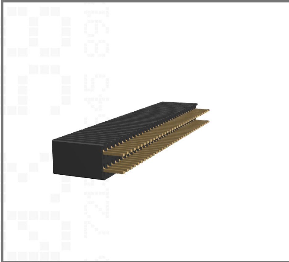
Dual row, 8.5mm high, gold, 36+36 contacts
