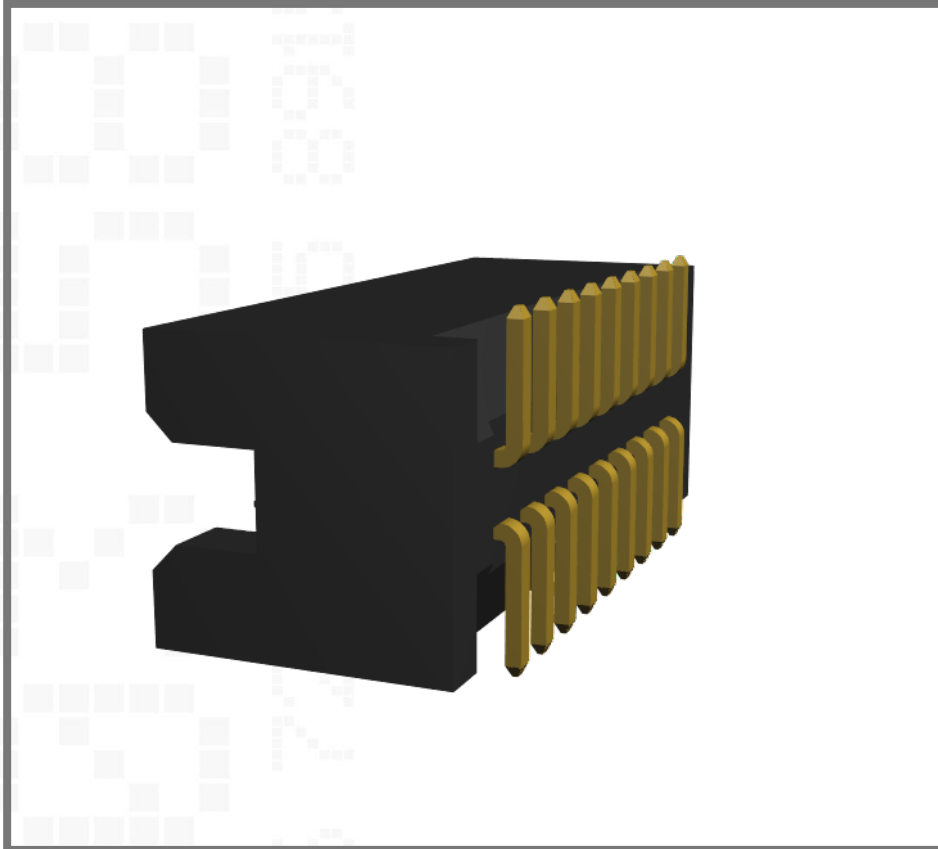
Dual row, Shrouded, 6.1mm high, Gold, 9+9 contacts
