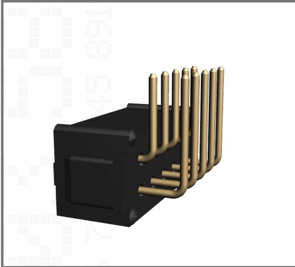
Double row, Unlatched, 3mm tail, Gold, 5+5 contacts
